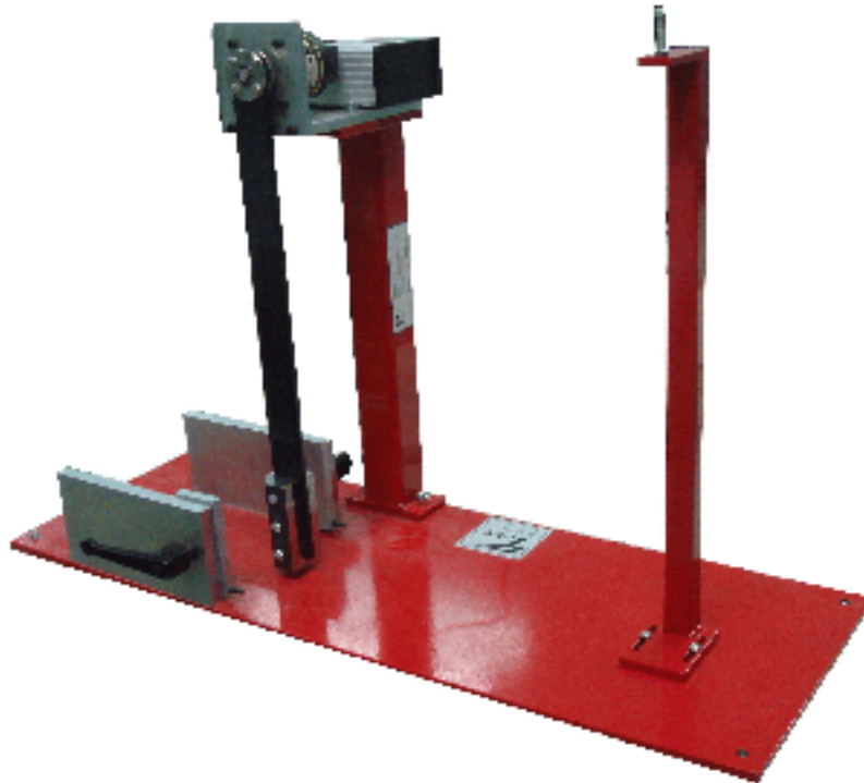
Pendulum Impact Tester 4J
