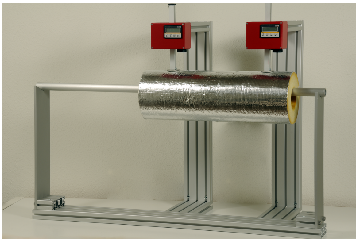
MTG-Pipe
